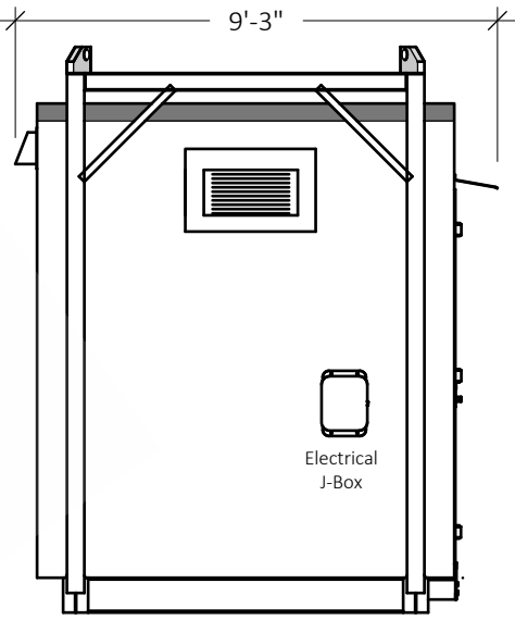
WEST VIEW EXTERIOR ELEVATION
