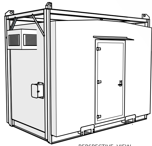
PERSPECTIVE VIEW EXTERIOR ELEVATION
