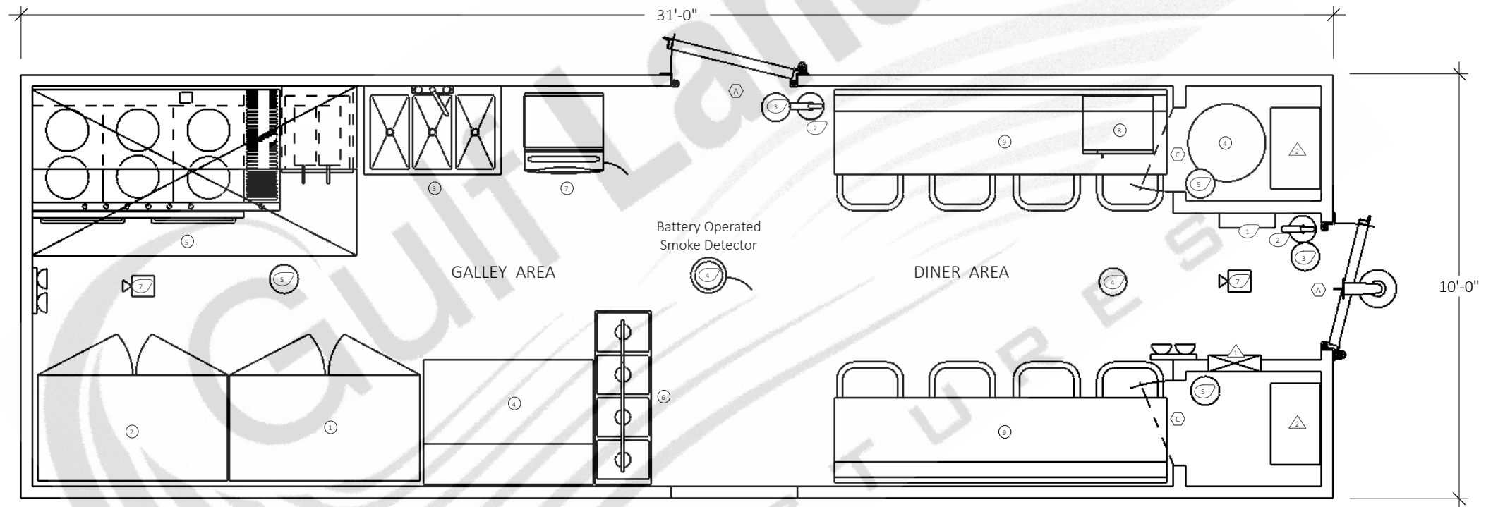
10' x 31' GALLEY / DINER
